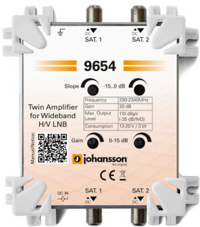
Ref. 9654 Wideband Trunk Amplifier
