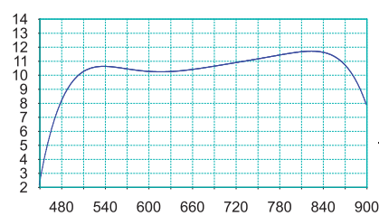
Gain (x: frequency MHz, y: ISO dBi gain) and Pattern (@862MHz)
