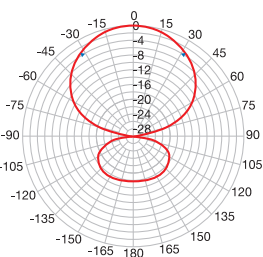
Gain (x: frequency MHz, y: ISO dBi gain) and Pattern (@200MHz)
